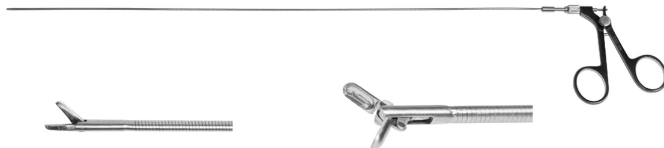
JP3003RB microscissors semi-rigid 5Fr \times 400mm
